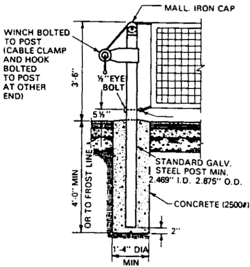
Figure 5.24 Tennis net and post details.
