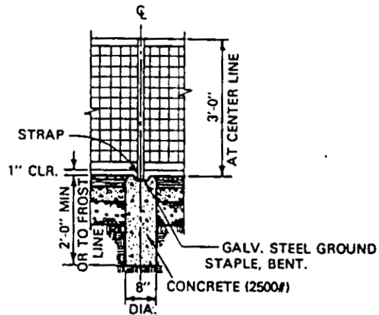
Figure 5.25 Anchor footing.
