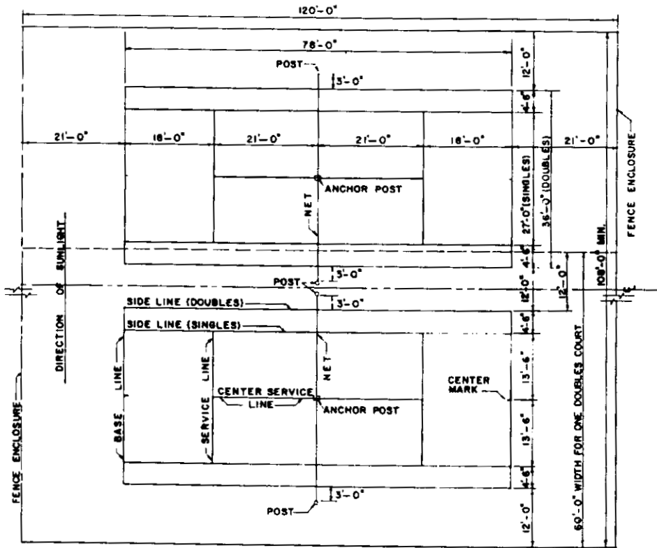
Figure 5.23 Tennis courts.
