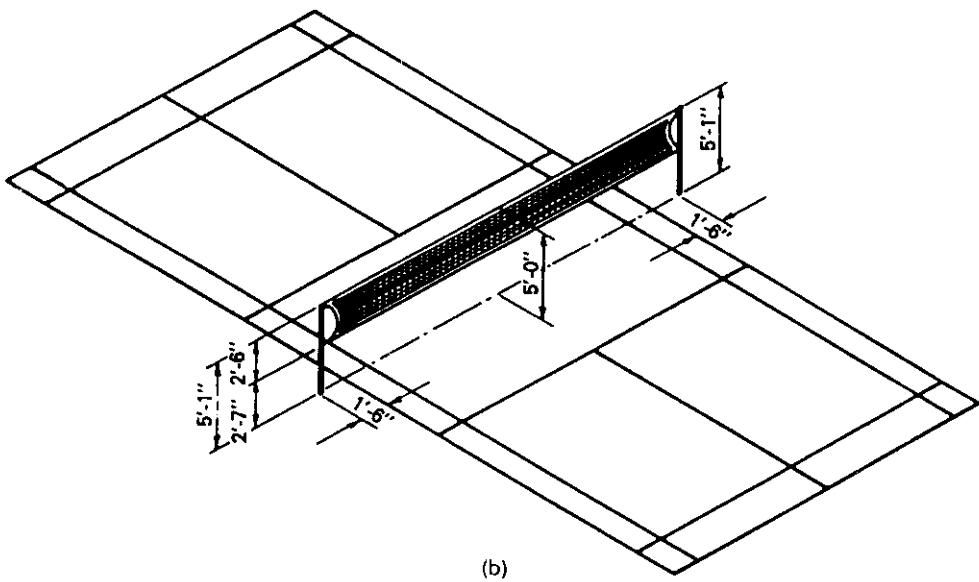
Figure 5.26 Badminton: (a) court layout; (b) isometric showing net.
