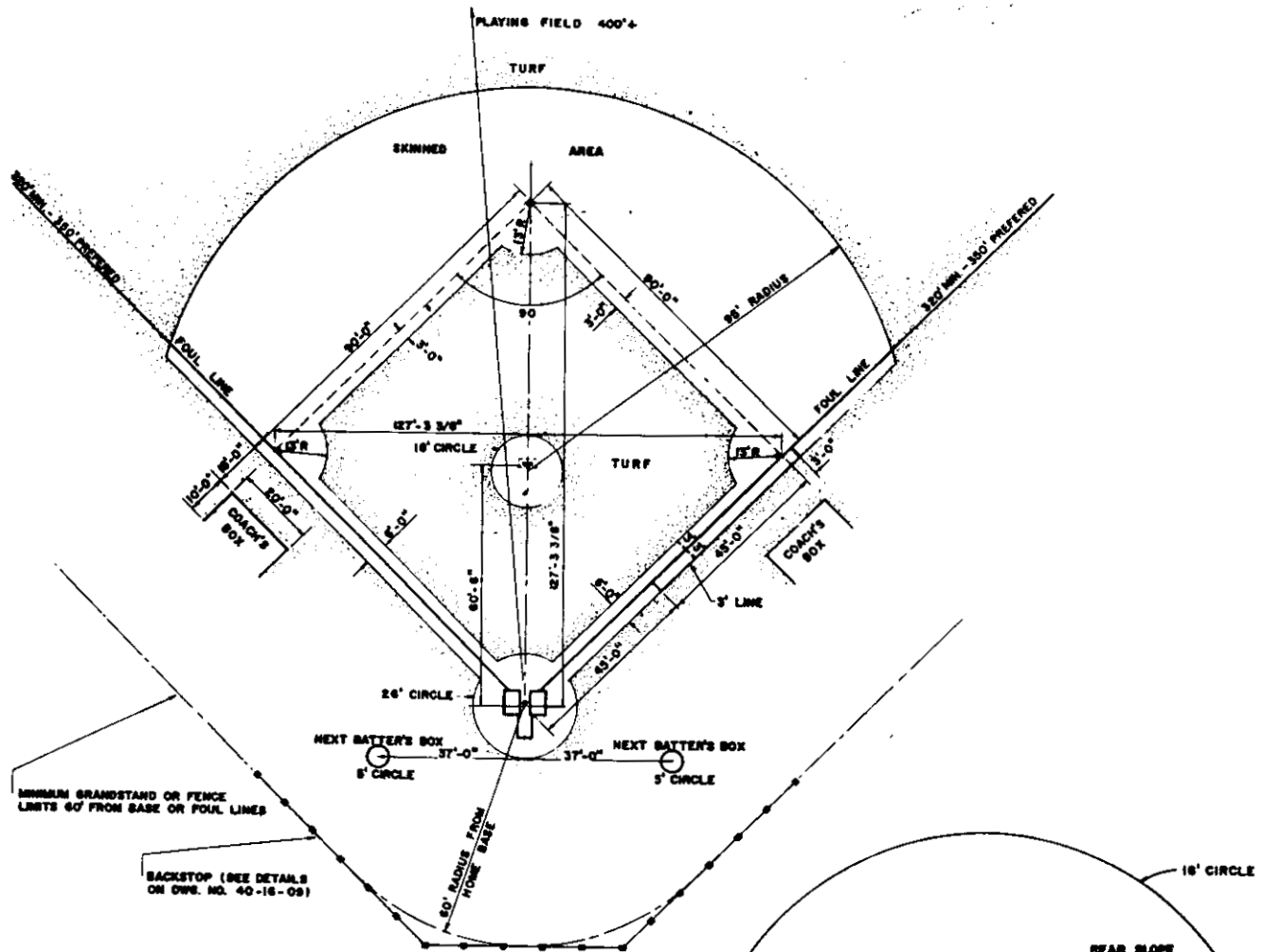
Figure 5.9 Baseball diamond.
