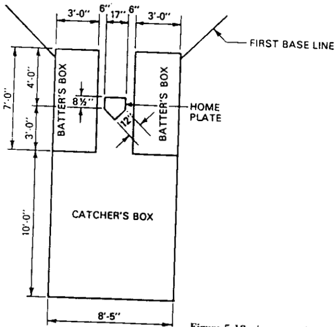
Figure 5.18 Layout at home plate.
